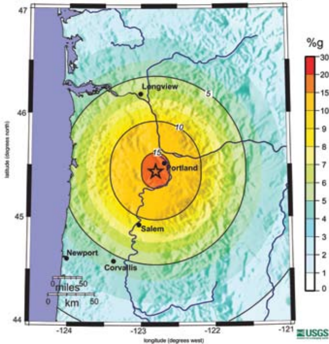
M6.5 'Beaverton' Earthquake, Depth 30 mi (50 km)
