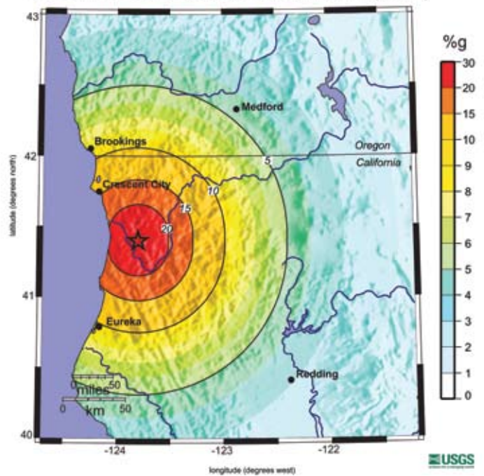
M6.8 'NW California' Earthquake, Depth 25 mi (40 km)
